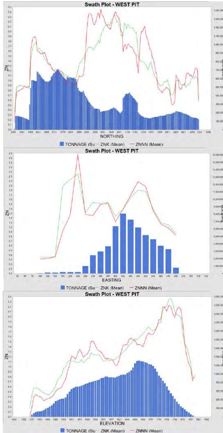
Figure 14-15 Swath Plots – Zn – West Pit
