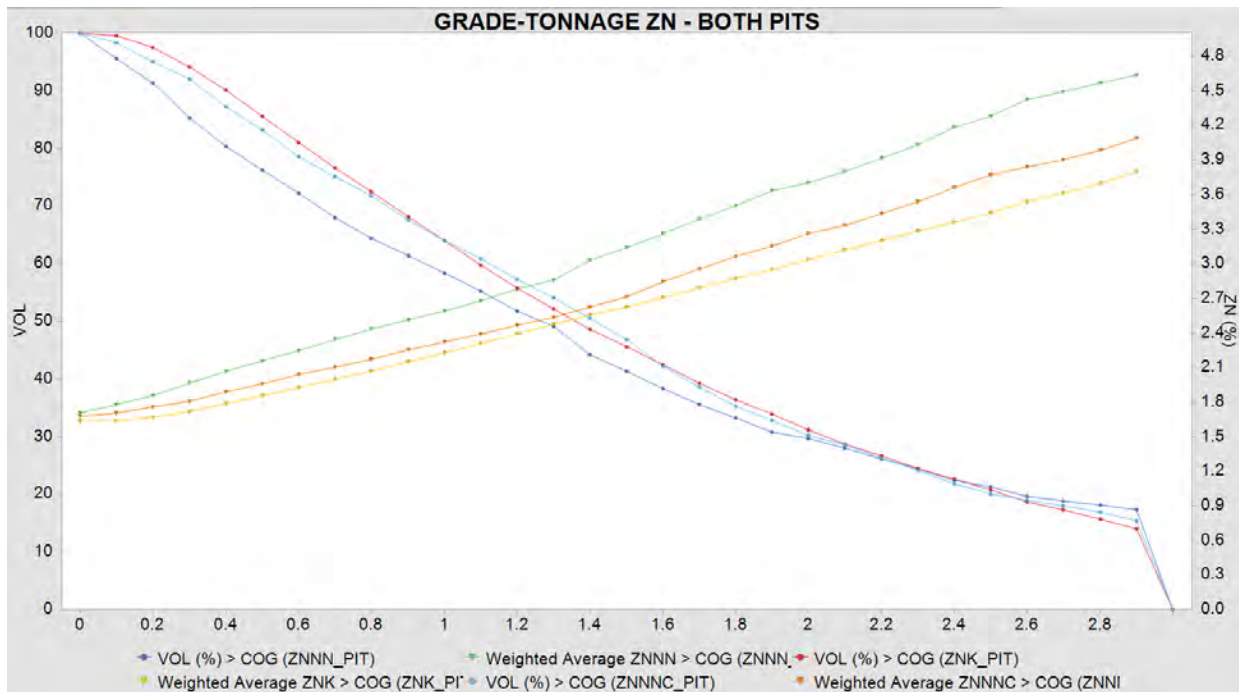
Figure 14-18 Grade-Tonnage Curves – Zn
